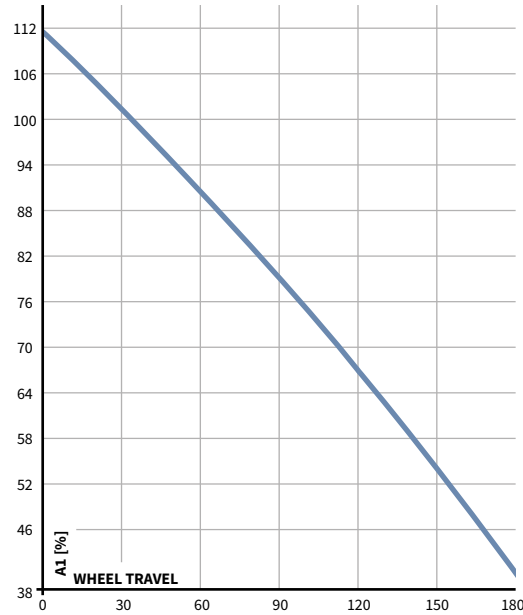
ANTI-SQUAT (34/24)
